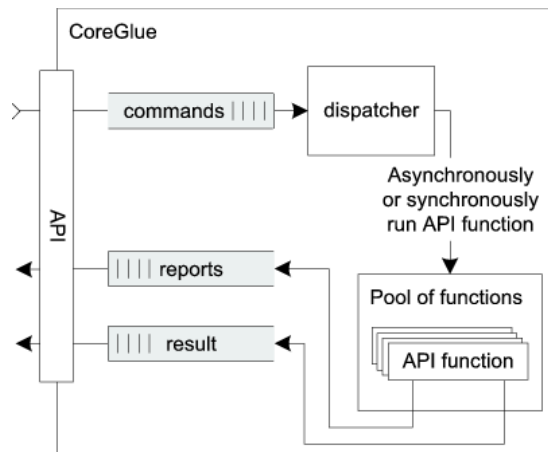
Figure 7: API and CoreGlue interaction.
