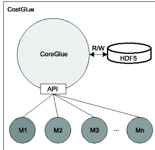
Figure 6: CostGlue architecture.
