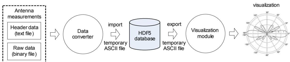
Figure 11: Import, export and visualization process of the antenna measurements results
