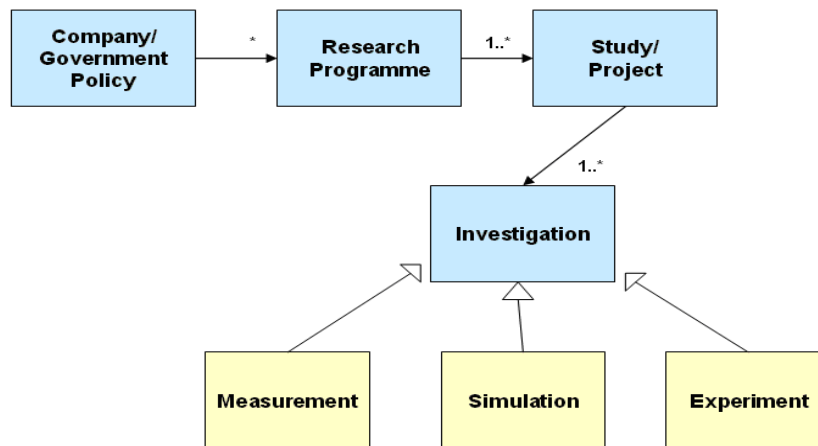
Figure 5: Main classes of the CSMD model version 2
