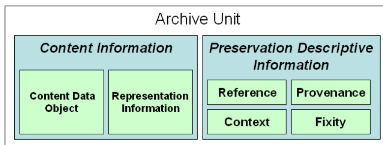
Figure 4: Archive package as defined in the OAIS information model
