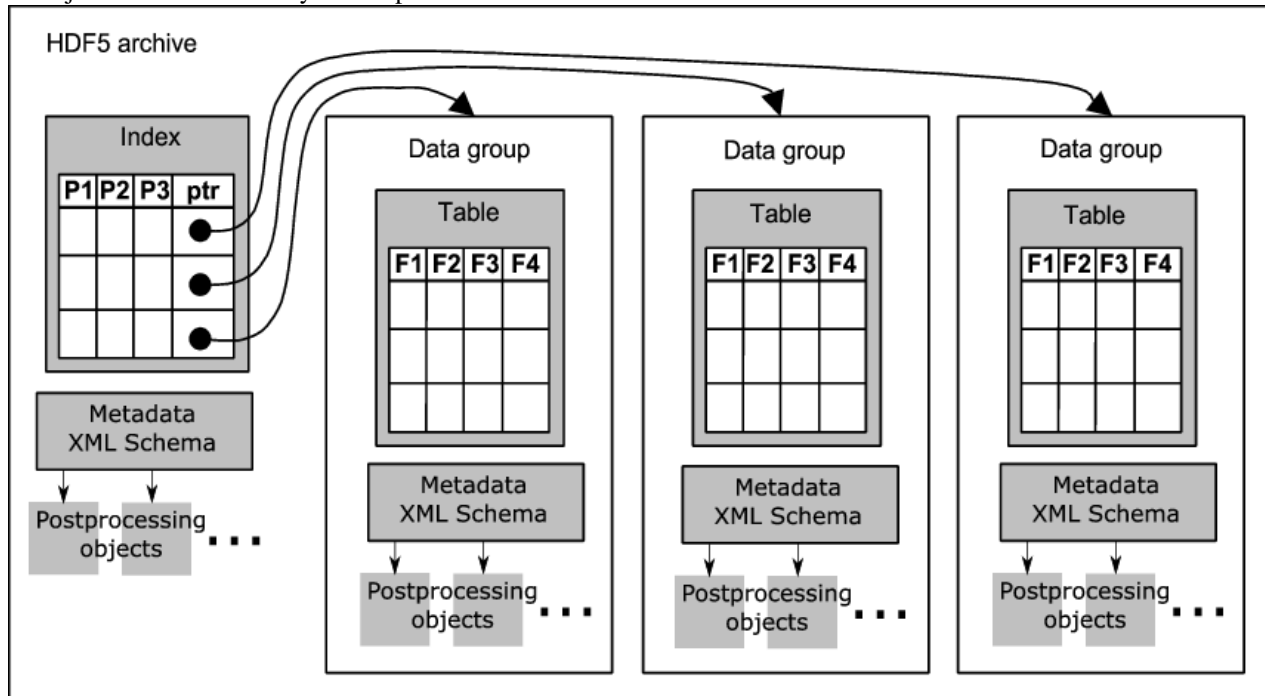
Figure 2: The logical structure of the database.
